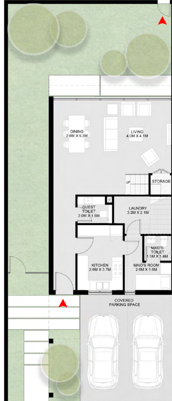
Ground Floor
