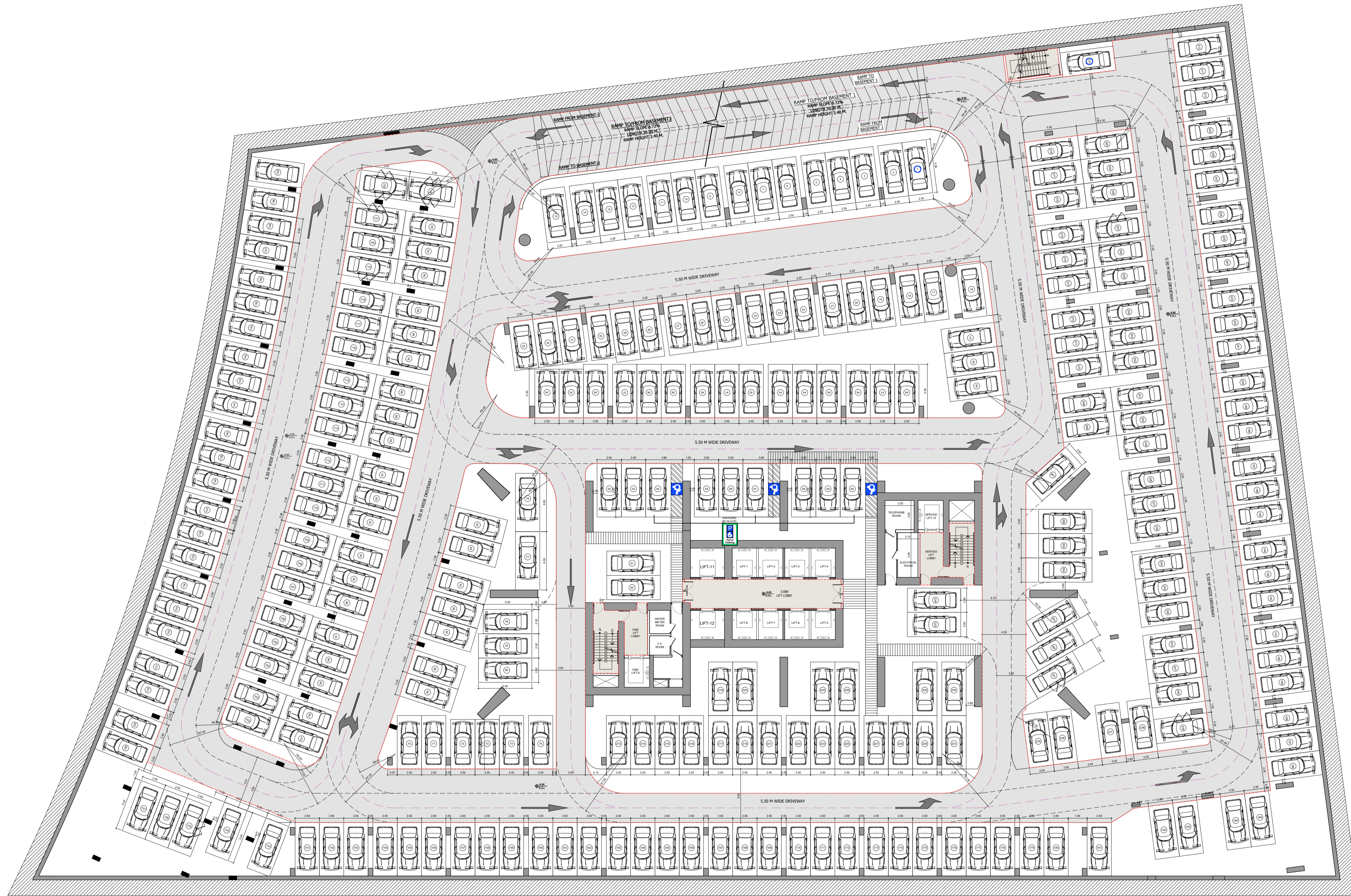
BASEMENT-2= 279 NOS. PARKING
